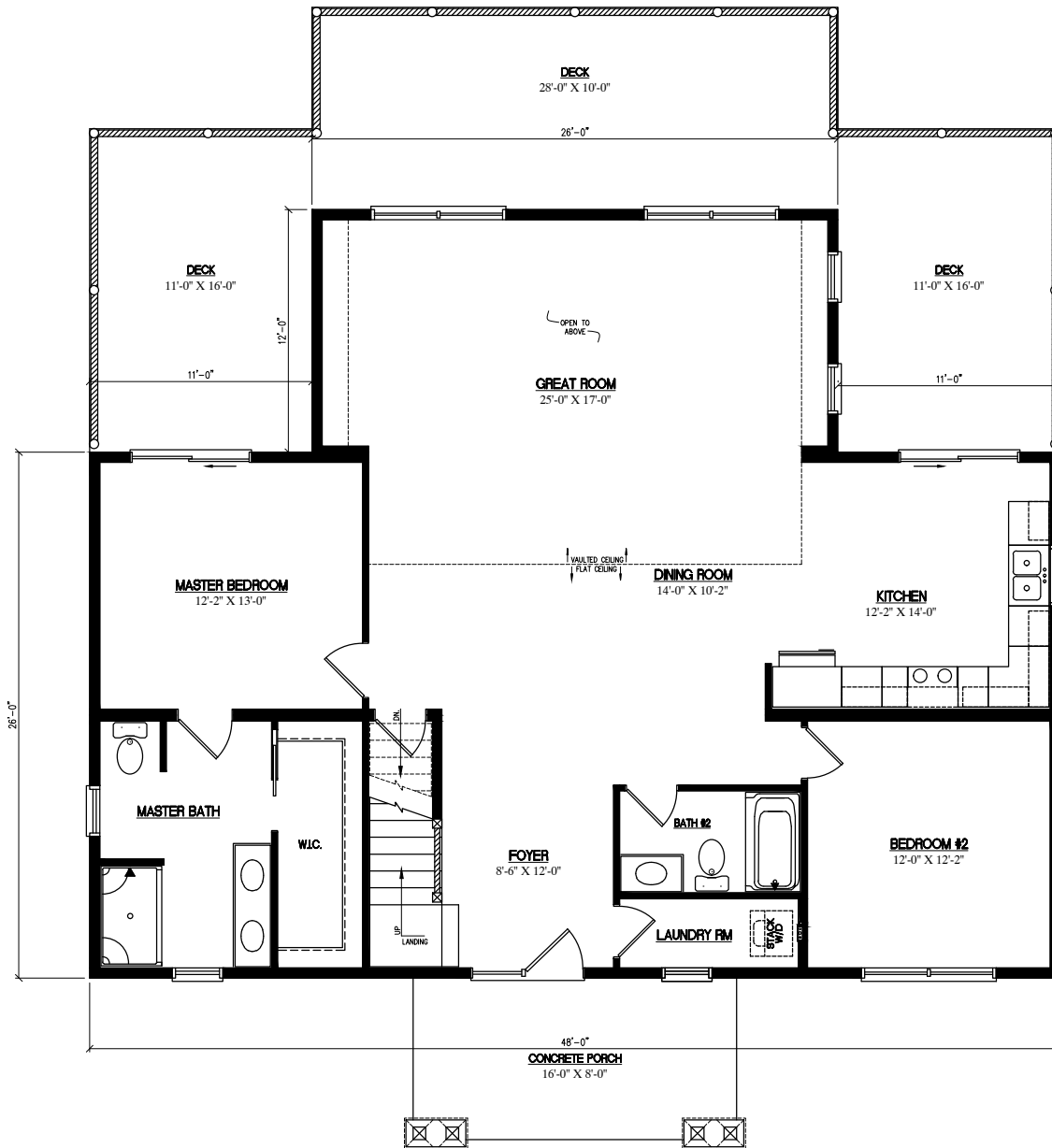
26' x 48' CANYON LODGE FIRST FLOOR 1560 SQ.FT.
