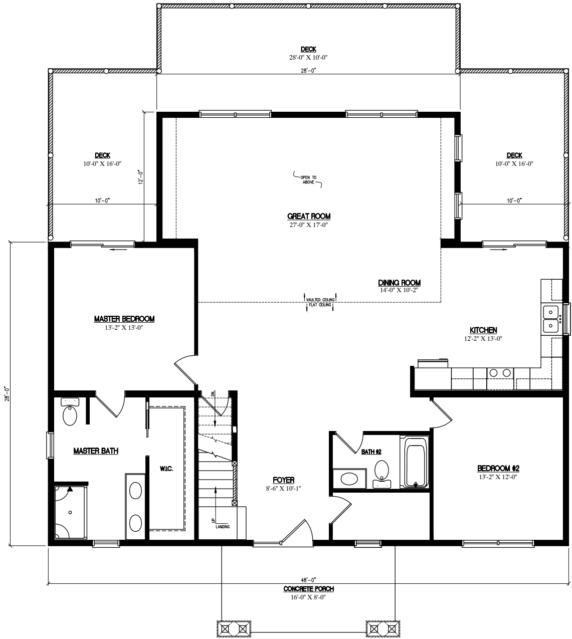
28' x 48' CANYON LODGE FIRST FLOOR 1680 SQ.FT.
