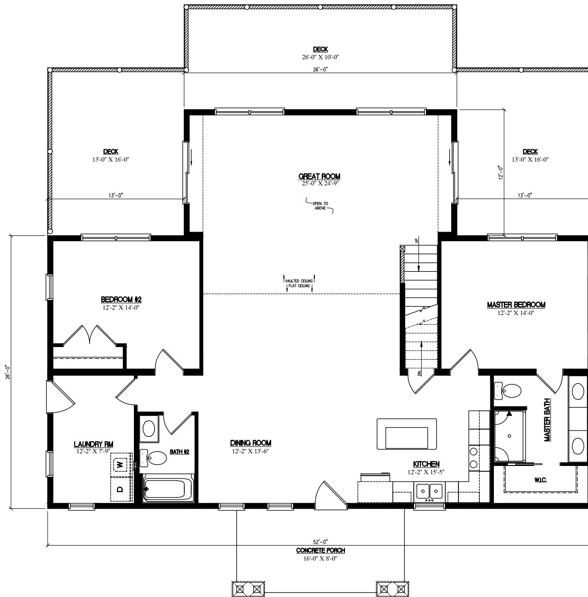
26' x 52' CANYON LODGE FIRST FLOOR 1664 SQ.FT.
